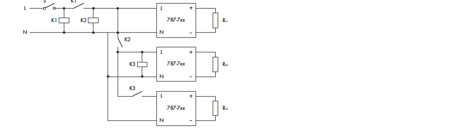
Fig. 3: Connecting power supply units in parallel
