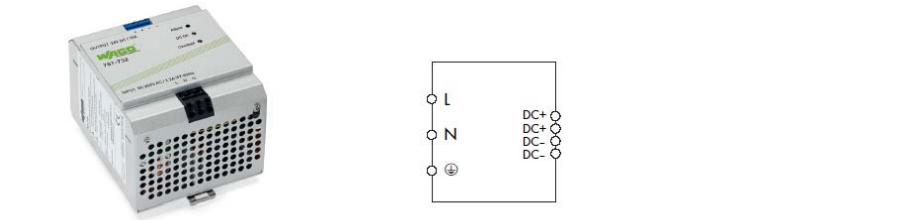
Fig. 1:787-732 Primary Switch DC Power Supply Unit
