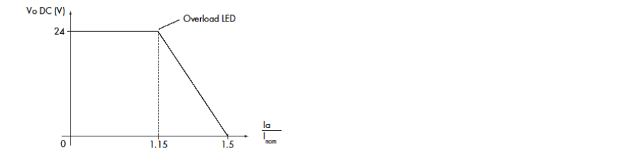
Fig. 4: Output characteristics
