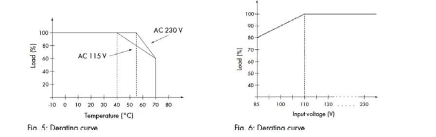
Fig. 5: Deratting curve
