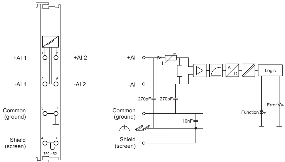
Fig. 2.1.1-3: 2-Channel Analog Input Module 750-452
