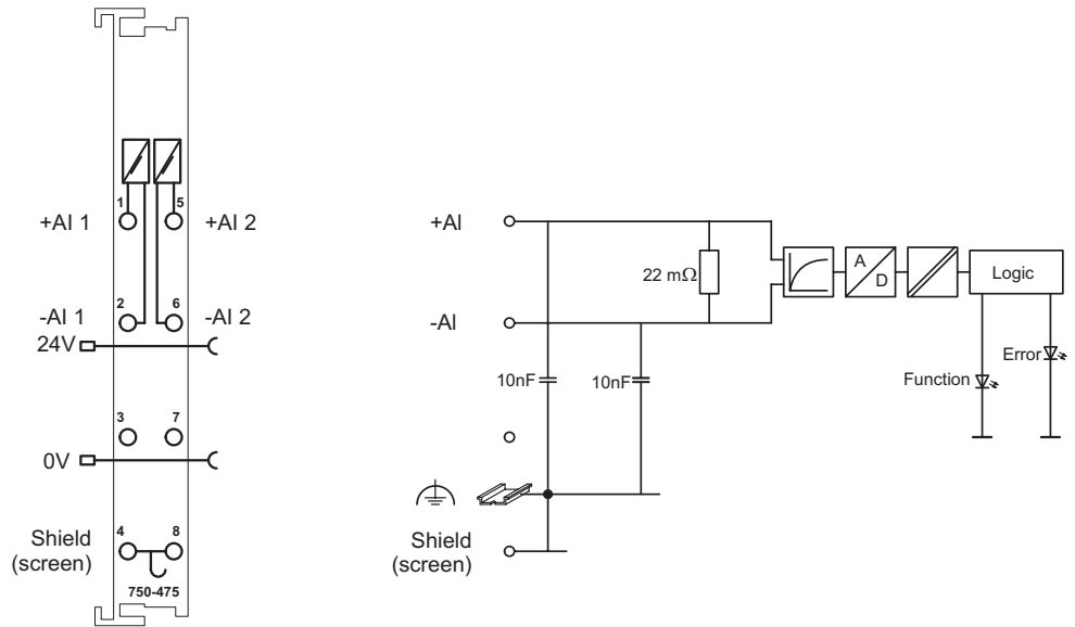
Fig. 2.1.1-3: 2- Schematic diagram
