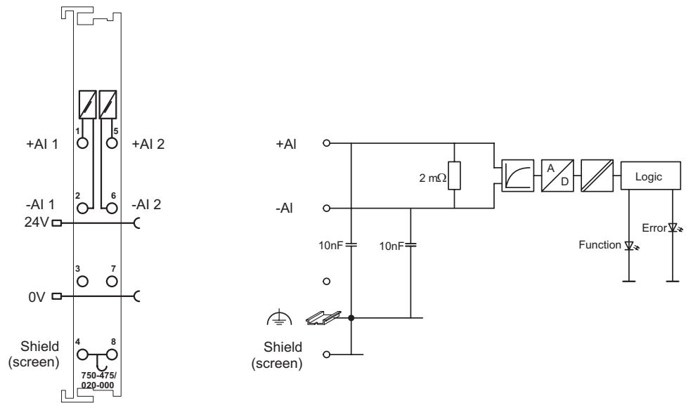
Abb. 2.1.1-3: 2 Schematic diagram
