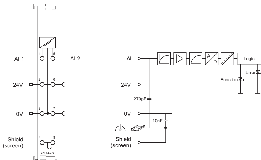
Fig. 2.1.1-3: 2-Channel Analog Input Module 750-478
