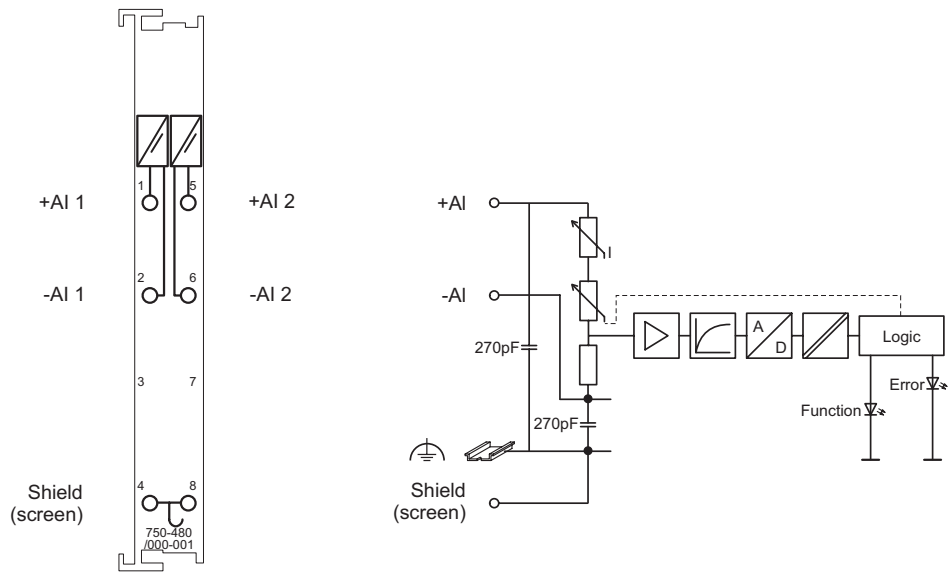
Fig. 2.1.2-3: 2-Channel Analog Input Module 0-20 mA
