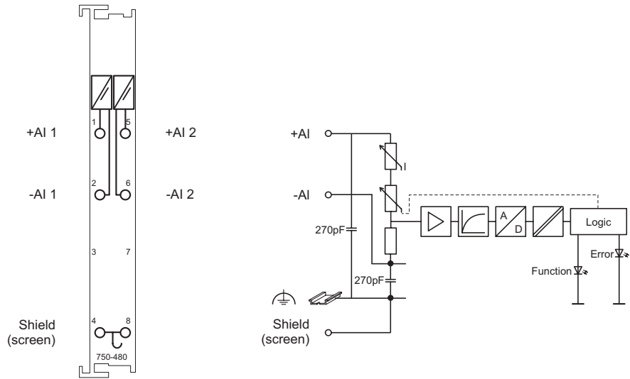
Fig. 2.1.1-3: 2-Channel Analog Input Module 0-20 mA
