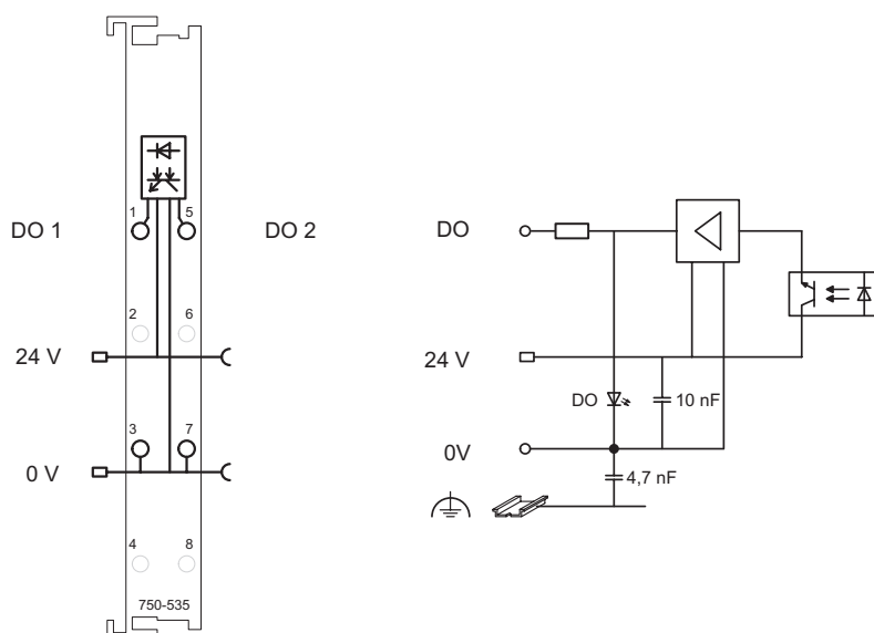
Fig. 2.1.1-3: 2-Channel Digital Output Module 750-535
