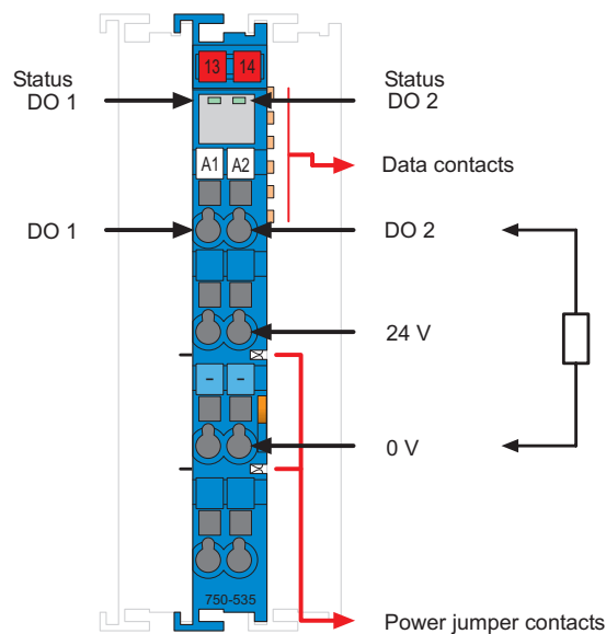
Fig. 2.1.1-1: 2-Channel Digital Output Module 750-535
