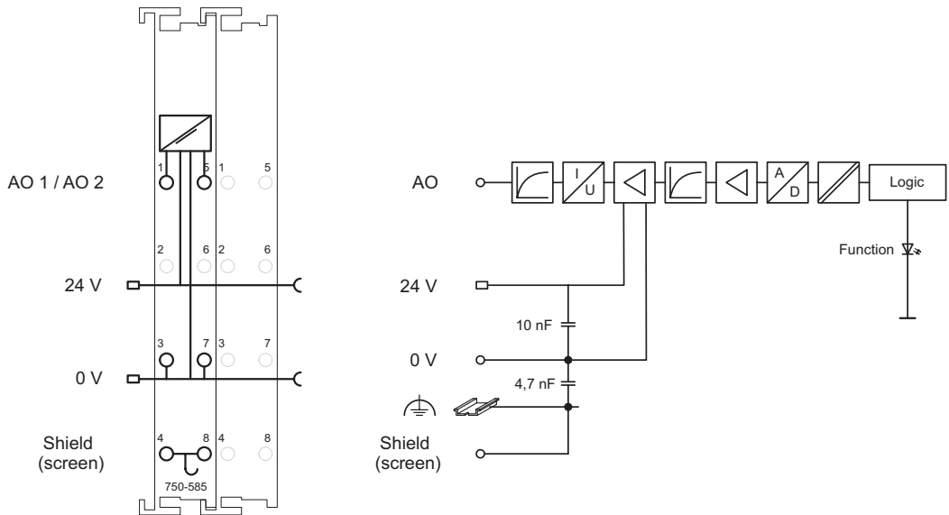
Fig. 2.1.1-3: 2-Channel Analog Output Module 750-585
