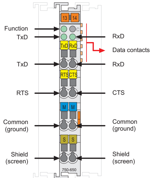
Fig. 2.1.1-1: Serial Interface 750-650
