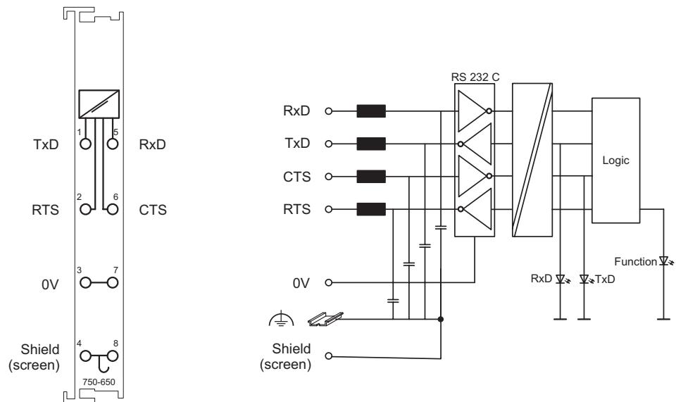
Fig. 2.1.1-3: Serial Interface 750-650
