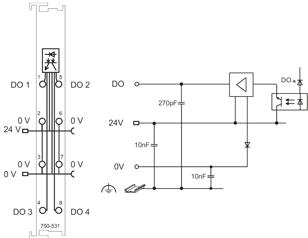
Figure 5: Circuit Diagram, HW 13 and Above ...
