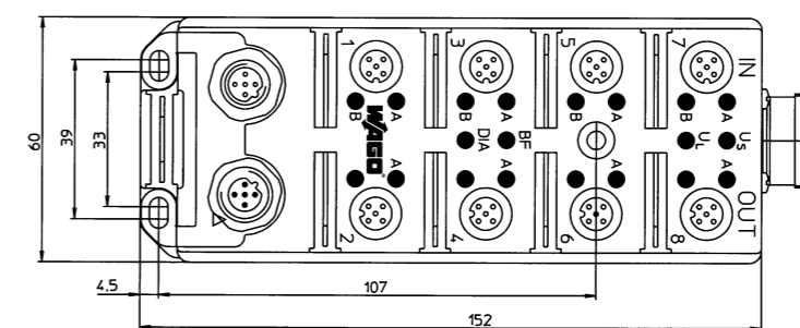
Montagemaße (mm) Dimensions (mm)
