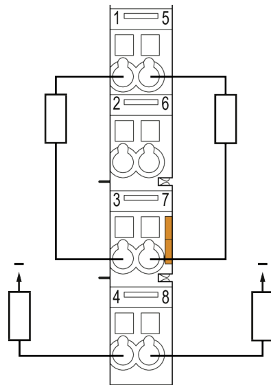
Figure 6: 2-Wire Connection
