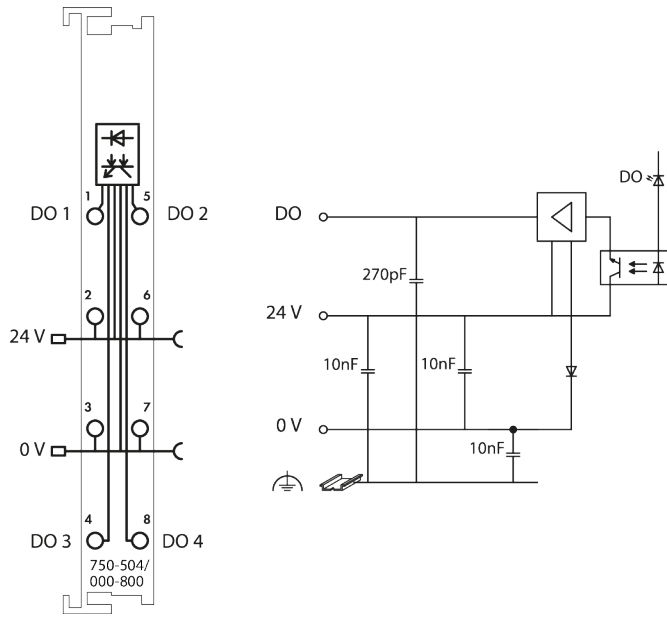
Figure 5: Schematic Circuit Diagram (Hardware Version 12 or higher)
