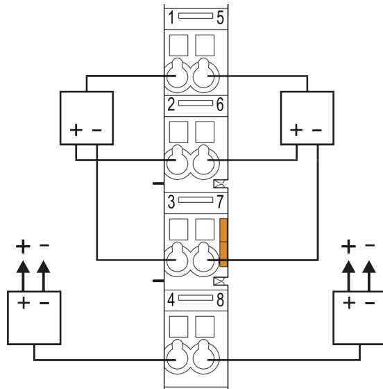
Figure 7: 3-Wire Connection
