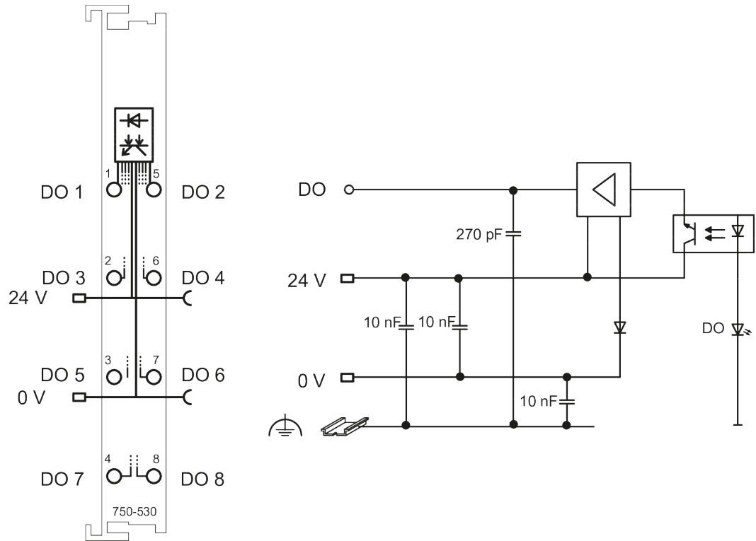
Figure 5: Circuit Diagram
