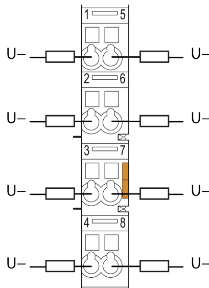
Figure 6: Connection Example
