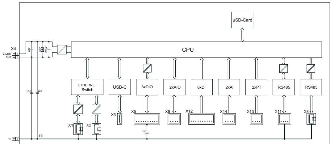
Figure 7: Circuit Diagram
