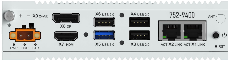
Figure 1: Front view
