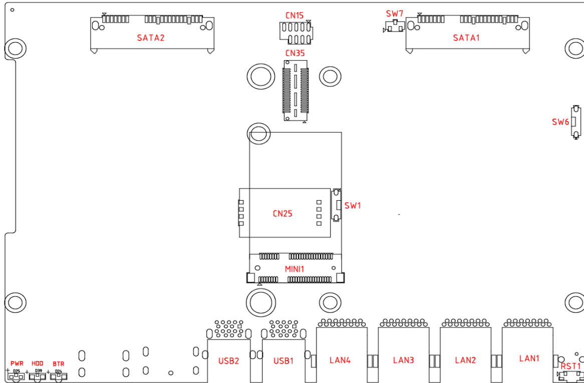
Figure 3: Circuit Diagram – SATA/mPCIe side
