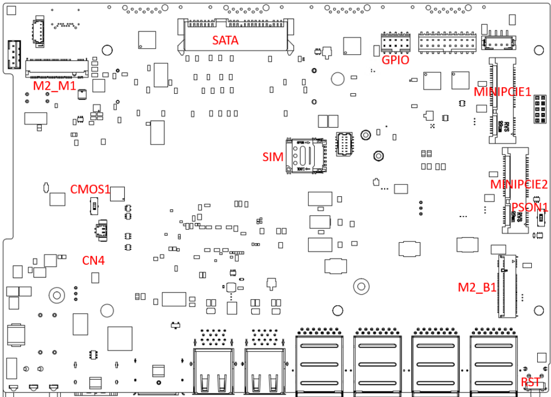
Figure 3: Circuit Diagram (bottom)
