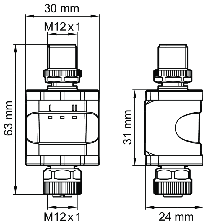
Figure 4: Dimensional Drawings
