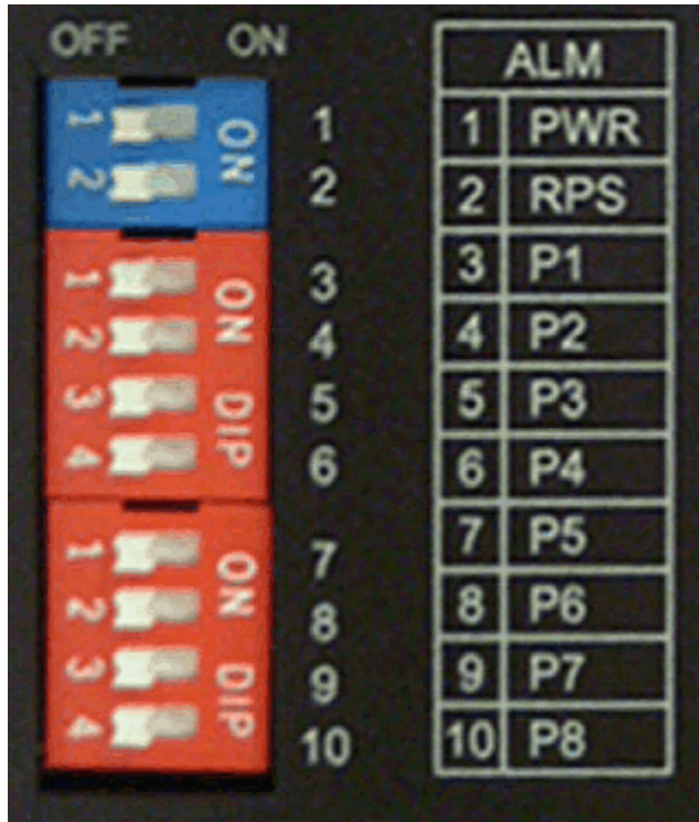
Figure 6: DIP switch
