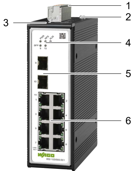
Figure 1: Front View
