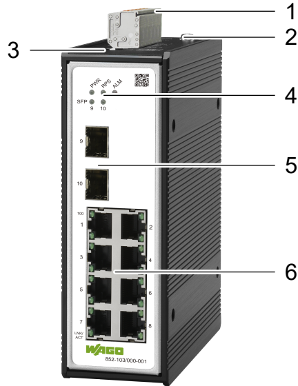
Figure 1: Front View
