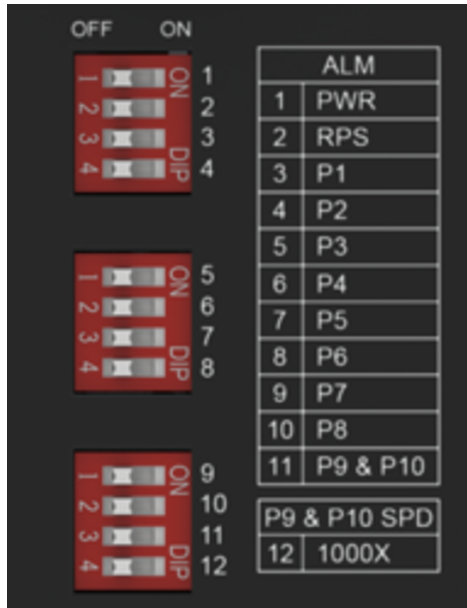
Figure 6: DIP switch
