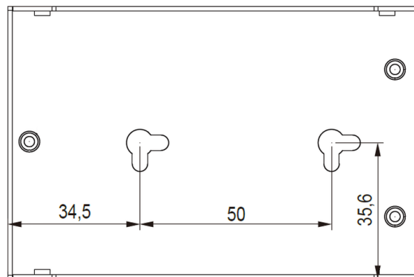
Figure 10: Dimensions of the Mounting Holes
