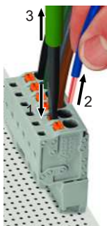
Figure 11: Removing Conductor from Push-in CAGE CLAMP®
