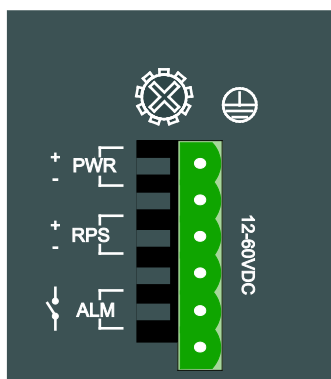
Figure 3: Power Supply (PWR/RPS)
