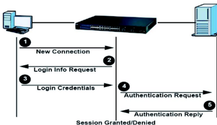
Figure 26: RADIUS Server
