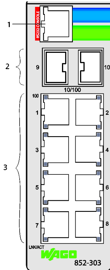
Figure 4: Network Connections
