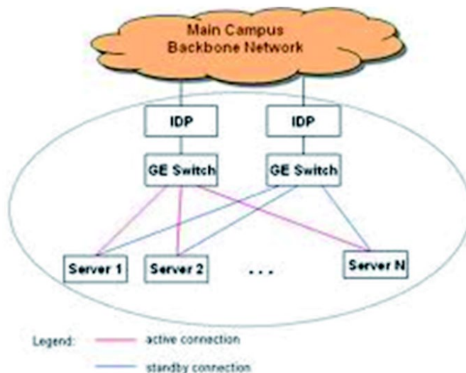
Figure 22: Dual Homing
