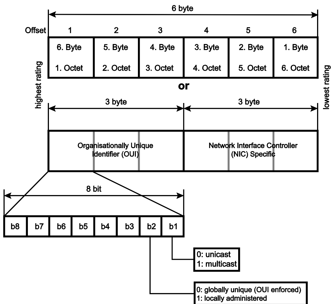
Figure 15: Multicast Address
