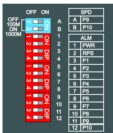
Figure 7: DIP Switches (Example)
