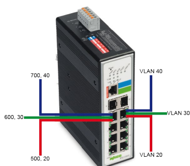
Figure 17: Configuration Example
