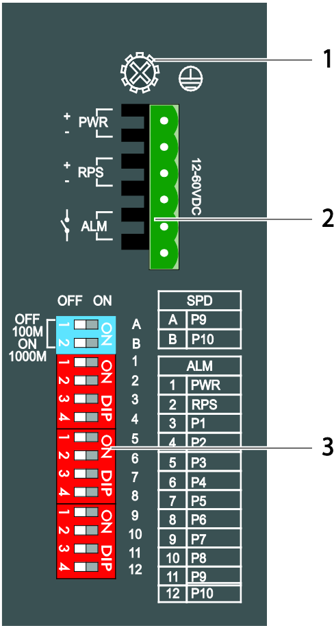
Figure 2: Top View of the Industrial Managed Switch (Example)
