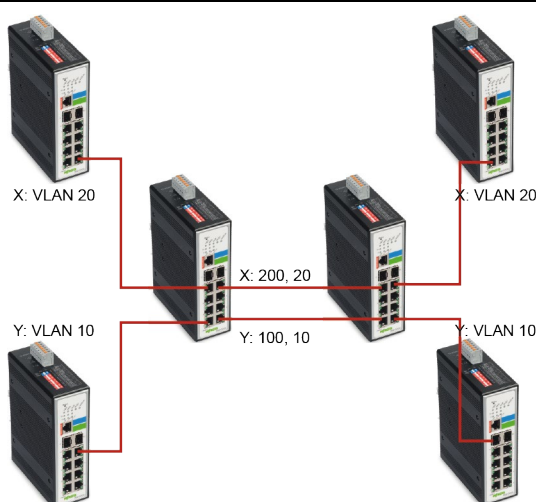
Figure 16: Port-Based Q-in-Q
