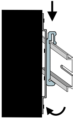
Figure 10: Removing the Device from the DIN Rail
