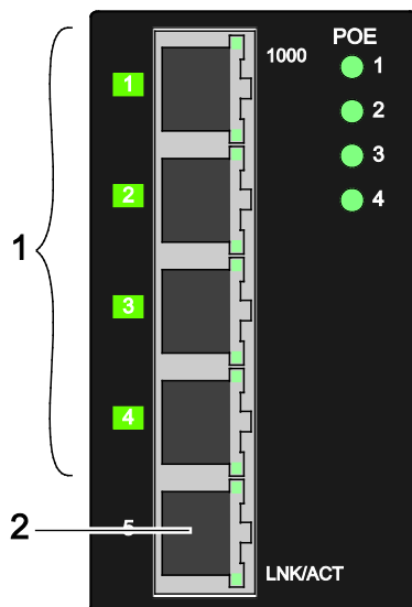
Figure 5: Network Connections
