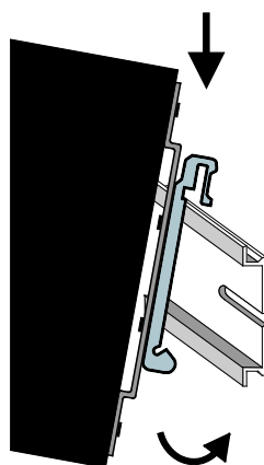
Figure 9: Snapping onto the DIN Rail
