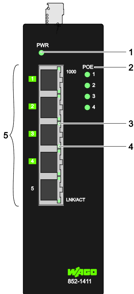
Figure 1: Front View of the Industrial ECO Switch
