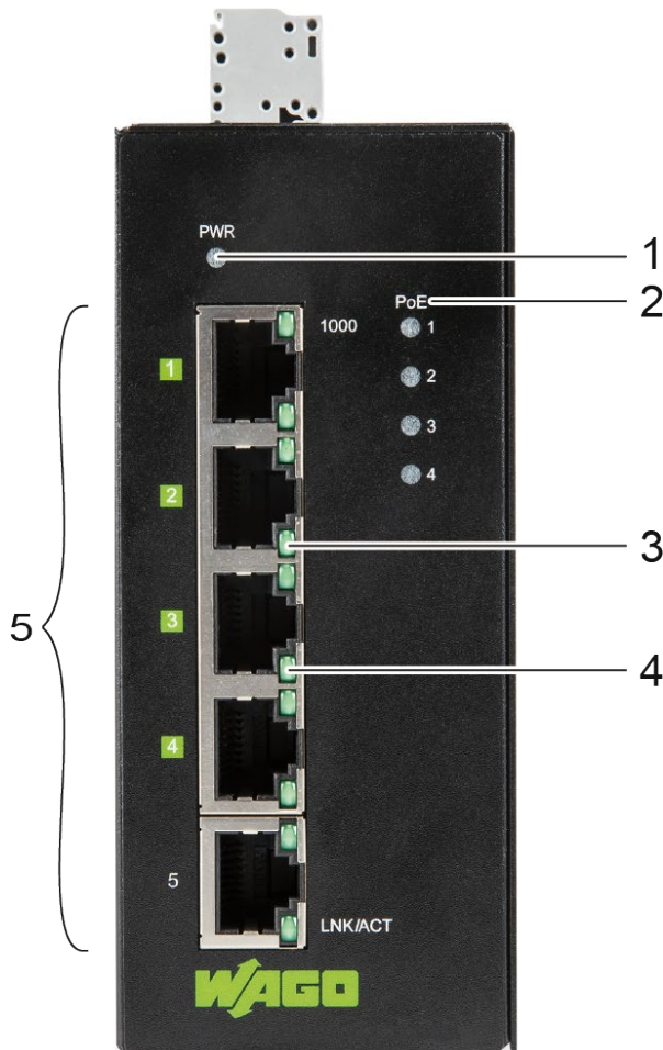
Figure 1: Front View of the Industrial ECO Switch
