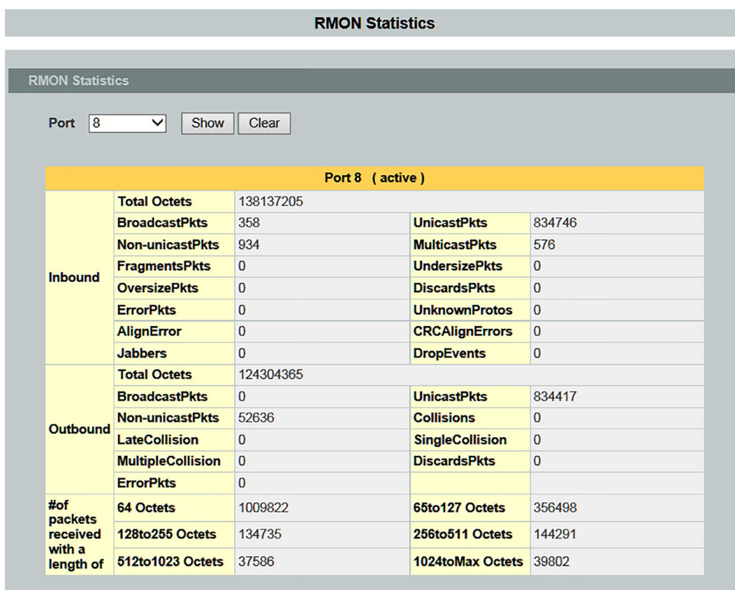
Figure 115: WBM “RMON Statistics” Page
