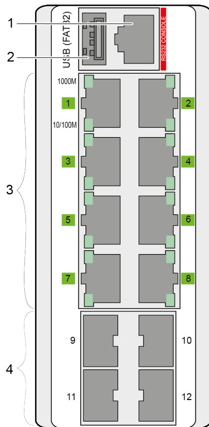
Figure 5: Network Connections
