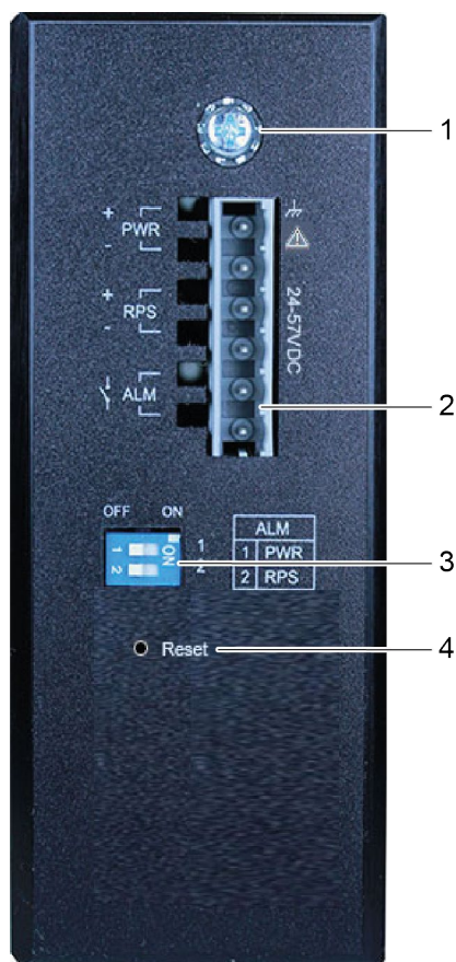
Figure 2: Top View of the Industrial Managed Switch
