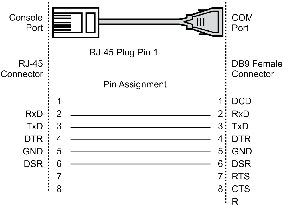
Figure 138: Connector Pin Assignment RJ-45 to DB9
