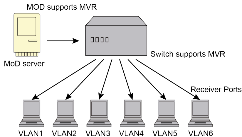
Figure 15: MOD Supports MVR
