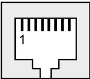
Figure 137: RJ-45 Connector Pin Assignment
