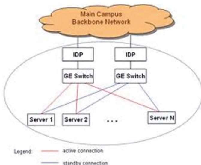
Figure 21: Dual Homing
