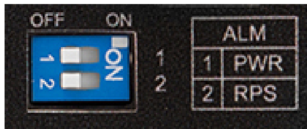
Figure 8: DIP switch
