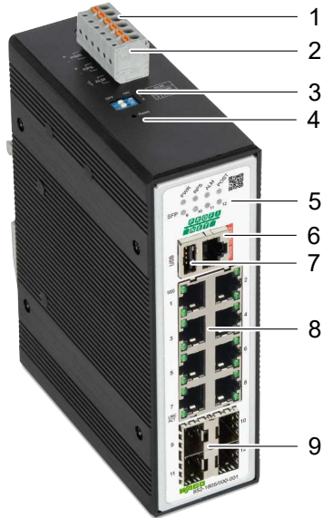
Figure 1: Front View
