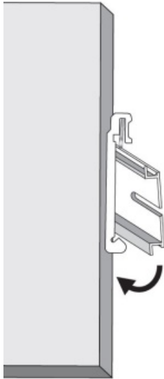
Figure 7: Removing the Product from the DIN-Rail
