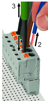
Figure 9: Removing Conductor from Push-in CAGE CLAMP®
