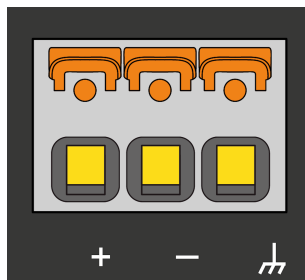
Figure 4: Power supply connection
