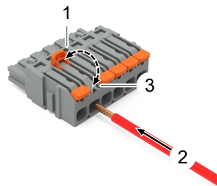
Figure 14: Connecting Conductor to Push-in CAGE CLAMP®
