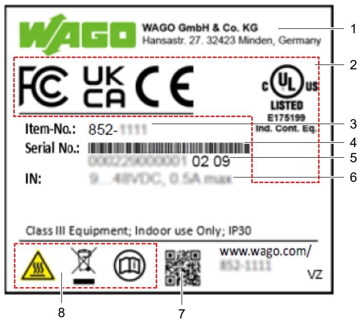
Figure 3: Type Plate (Example)
