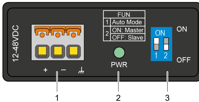
Figure 2: View from above
