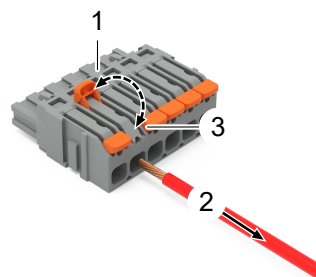
Figure 15: Removing Conductor from Push-in CAGE CLAMP®
