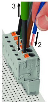
Figure 10: Connecting Conductor to Push-in CAGE CLAMP®
