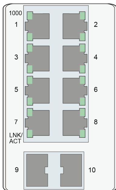
Figure 7: Port LEDs
