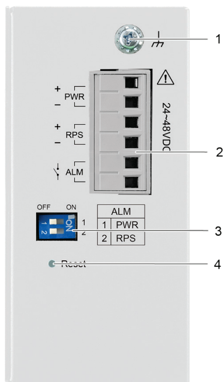
Figure 2: Top View of the Lean Managed Switch
