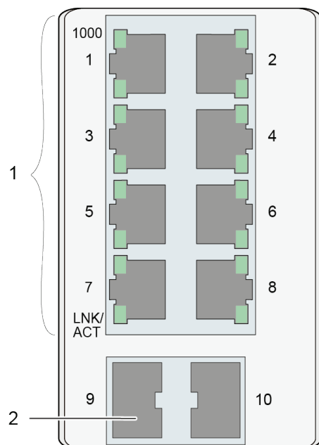
Figure 5: Network Connections
