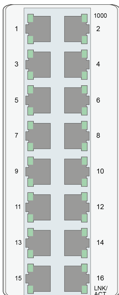
Figure 7: Port LEDs
