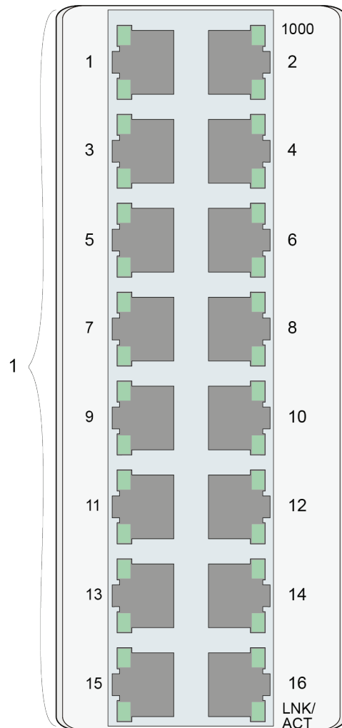
Figure 5: Network Connections
