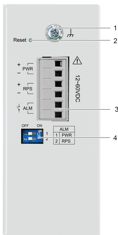
Figure 2: Top View of the Lean Managed Switch
